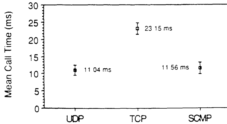
Fig. 5. Performance when clients make occasional calls to a server.
