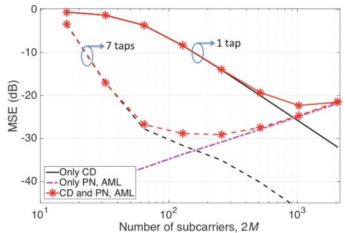
Fig. 8. Trade-off between the CD and PN compensation, 1000 km fiber and 400 kHz linewidth. Black solid lines: 1 tap equalizer; Black dashed lines: 7 taps equalizer.
