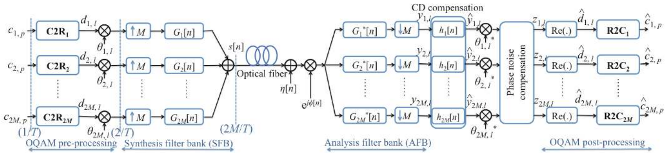
Fig. 1. FBMC/OQAM system model, considering the chromatic dispersion and laser phase noise impairments.
