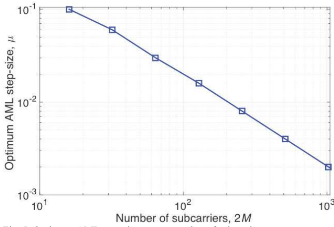
Fig. 5. Optimum AML step-size versus number of subcarriers.
