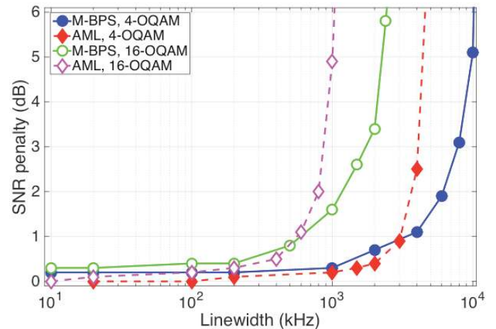
Fig. 10. SNR penalty at a BER of 10^{-3} versus laser linewidth after 1000 km transmission. 7-tap FS equalizer is used. Number of subcarriers: 2M = 256 .
