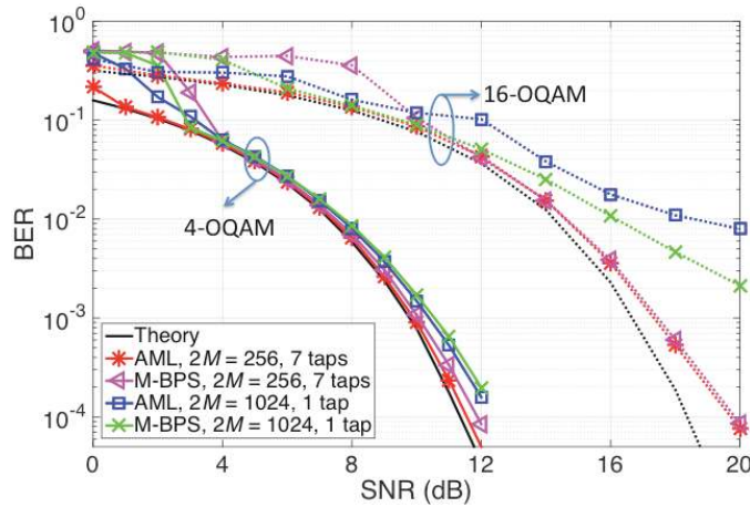
Fig. 9. BER versus SNR after 1000 km transmission with the combined laser linewidth of 400 kHz. Theory curves are achieved with only AWGN. Solid lines: 4-OQAM modulations; dotted lines: 16-OQAM modulations.
