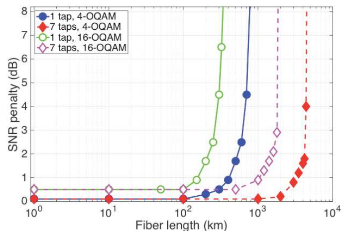
Fig. 11. SNR penalty versus fiber length at the 10^{-3} BER for 4- and 16-OQAM signals with laser linewidth \Delta\nu = 400 kHz and 2M = 256 .
