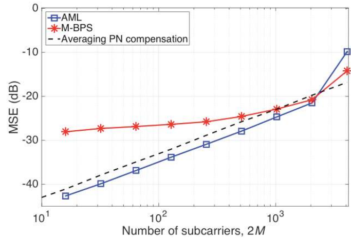
Fig. 6. MSE versus number of subcarriers using different PN compensation. Averaging PN compensation is carried out with the assumption of knowing PN.
