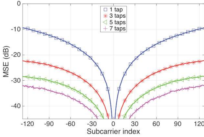
Fig. 3. MSE of the received symbols at each subcarrier index after a 1000 km optical fiber transmission, in the absence of PN and AWGN. 256 subcarriers are used.
