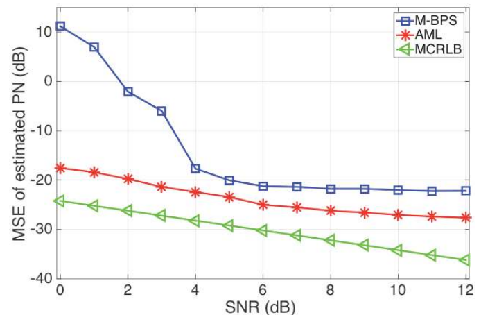
Fig. 7. MSE of the estimated PN versus SNR. Laser linewidth is set to 400 kHz and 2M = 256 .
