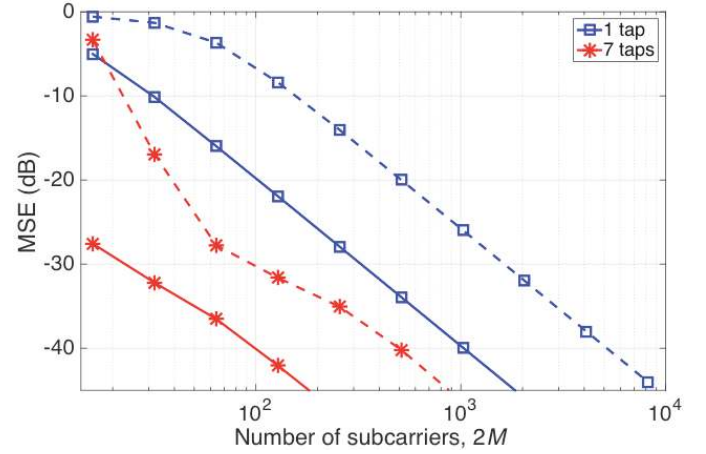
Fig. 4. MSE versus number of subcarriers, in the absence of PN and AWGN. Solid lines: 200 km, dashed lines: 1000 km.
