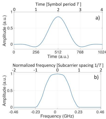
Fig. 2. Presentation of the prototype filter in a) time and b) frequency domains.
