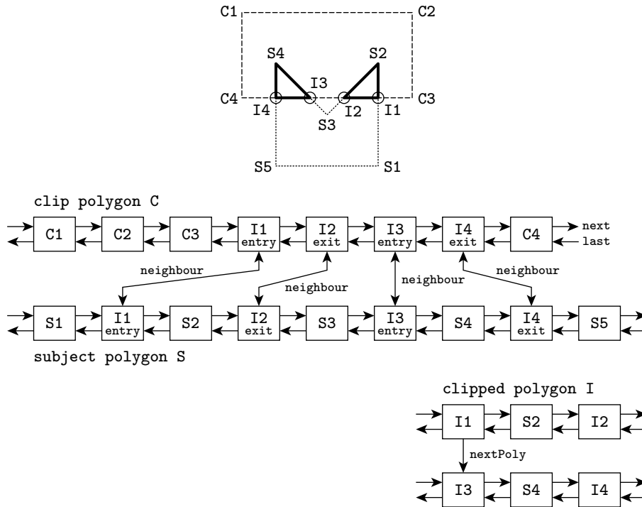
Figure 10: Data structure for polygons.
