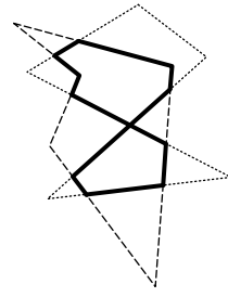
Figure 7: The resulting clipped polygon.
