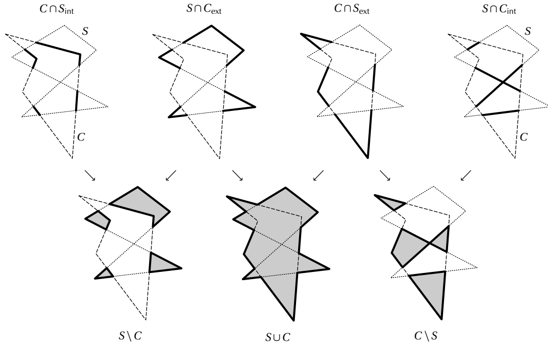
Figure 8: Set theoretic differences and union of two polygons.
