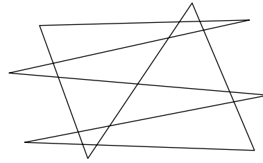
Figure 17: Worst case for self-intersection.
