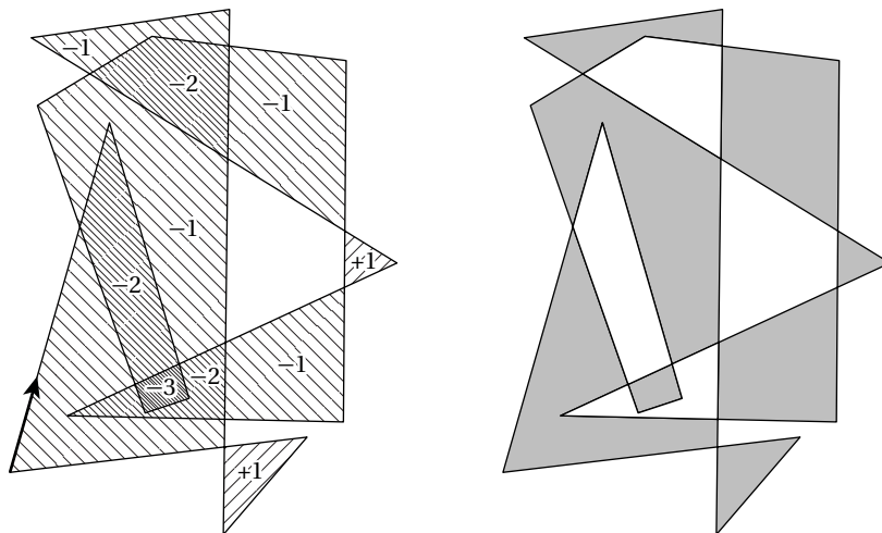
Figure 3: Winding numbers ( \neq 0 ) and interior for an arbitrarily complex polygon.
