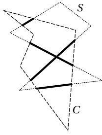
Figure 5: Parts of subject polygon inside clip polygon ( S \cap C_{int} ).
