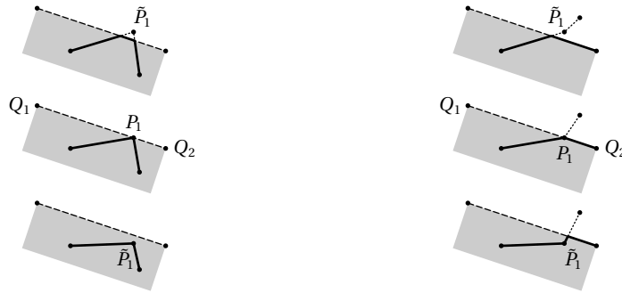
Figure 15: Two degenerate configurations (left/right); two possible perturbations for each example (upper/lower).
