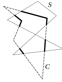
Figure 6: Parts of clip polygon inside subject polygon ( C \cap S_{int} ).
