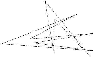
Figure 16: Worst case for the intersection of two polygons.
