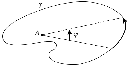
Figure 1: Winding number: \omega(\gamma, A) = \frac{1}{2\pi} \int d\varphi .
