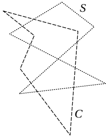
Figure 4: Example of clip polygon (C) and subject (S) polygon.
