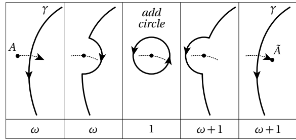
Figure 2: Change of the winding number when a point crosses the curve.
