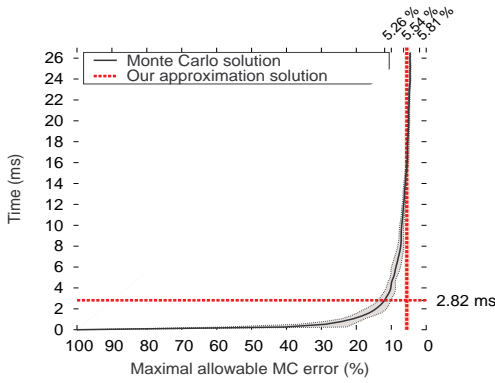
Figure 18: g_5, W_{cutoff} = \frac{1}{4}\alpha_i, K_{12} (W)
