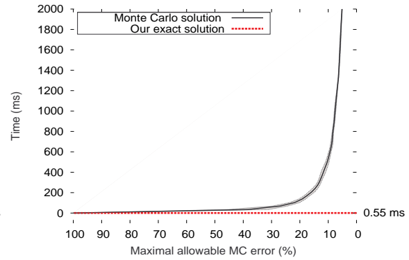
Figure 6: g_2 , k = 2 , WSPG (UW)
