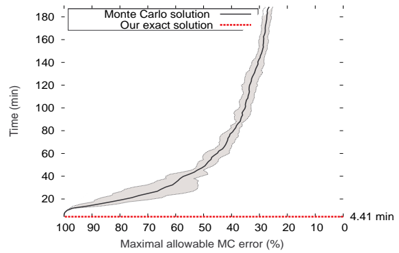
Figure 12: g_3, d_{cutoff} = \frac{d_{avg}}{4} , APhC (W)
