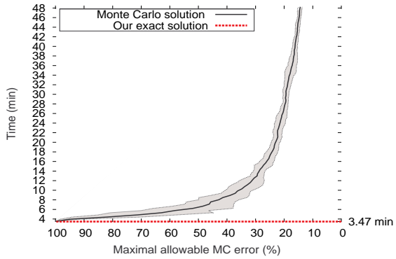
Figure 11: g_3, d_{cutoff} = \frac{d_{avg}}{8} , APhC (W)
