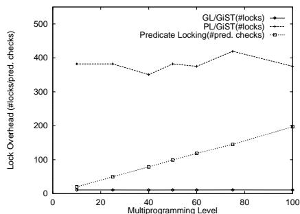
Figure 11: Lock Overhead of Search Operation (transaction size=10, write probability=0.2, query selectivity=0.1%)
