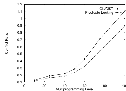
Figure 10: Conflict Ratio (transaction size=10, write probability=0.2, query selectivity=0.1%)
