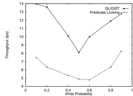
Figure 7: Throughput at various mixes of reads and writes (MPL=50, transaction size=10, query selectivity=0.1%)
