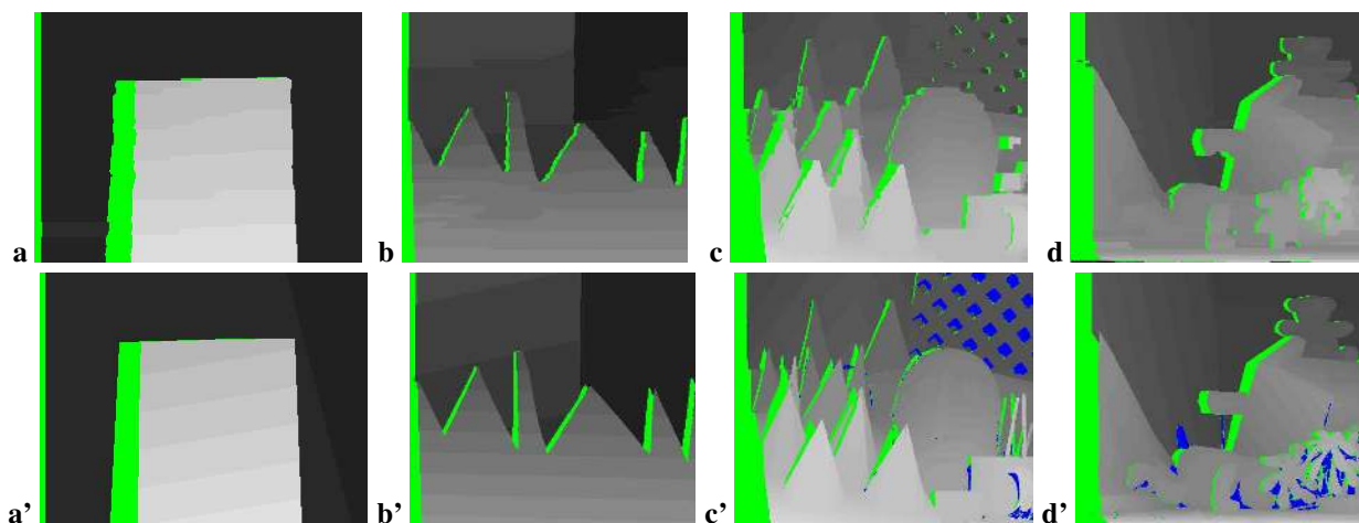
Fig. 18. Accuracy of occlusion estimation on the Middlebury stereo pairs. (a, · · ·, d) Estimated occlusions and disparities for the left view of Map, Sawtooth, Cones and Teddy stereo pairs, respectively. (a', · · ·, d') Corresponding ground-truth occlusions and disparities (blue pixels denote unlabelled pixels). Good correspondence between the ground-truth occlusions and those estimated by 4-state DP is evident. The maximum occlusion gap of 55 pixels (12% of image width) occurs at the edge of the Cones image. The maximum occlusion for Map is about 9% of the image width.
