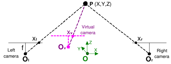
Fig. 25. Notation for virtual image generation. O_l , O_r and O_v are the optical centres of left, right and virtual cameras respectively. The optical centre of the virtual camera can be placed anywhere in space and the corresponding virtual image is synthesized by our algorithm.
