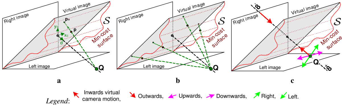
Fig. 26. Virtual camera motion. (a) The 3D motion of the virtual camera is achieved by direct projections of points on the minimum cost surface onto the virtual image plane. The reference coordinate system (x_c, y_c, d) has origin in the centre of the virtual image plane. (b) The virtual image is generated directly by projecting points from the minimum-cost surface S into the virtual image plane. (c) Moving the centre of projection Q corresponds to translating the virtual camera. The coloured arrows indicate the mapping between moving the centre of projection Q in our diagram and the corresponding translations of the virtual camera in the scene.
