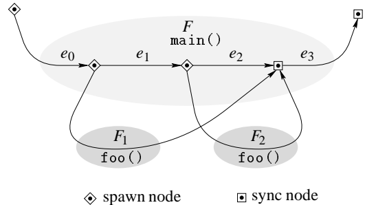
Figure 3: The parallel control-flow dag of the program in Figure 1. A spawn node of the dag represents a spawn construct, and a sync node represents a sync construct. The edges of the dag are labeled to correspond with code fragments from Figure 1. We assume that the start of the program is “spawned” by the operating system, and the end of the program is “synced” by the operating system.
