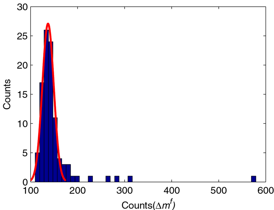
Figure 2 Frequency Distribution of high-frequency \Delta m ( \Delta m^f ) for data set 1. The random part of the distribution is very close to a Gaussian distribution, based on which the p -value of a \Delta m_i^f being random can be computed.
