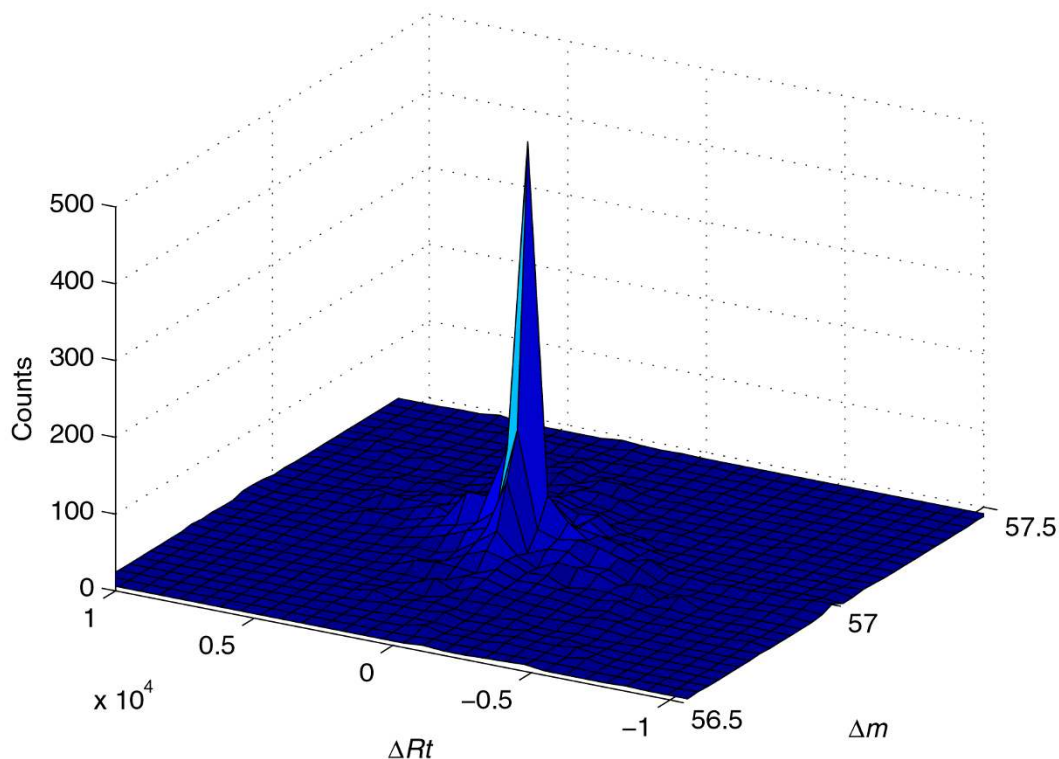
Figure 3 2-D histogram of \Delta m and \Delta Rt for the carbamidomethylation modification found in data set I. The sharp peak in both dimensions indicates the actual presence of this modification in the sample, since a modification must cause a fixed change in peptide mass and a slight shift in retention time.
