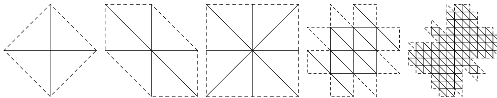
Figure 2: Stencil used in the classical Fast Marching algorithm (first), the AGSI [4] (second), the FM-8 (third), and the MAOUM [2] at a grid point z \in \Omega_* when the local anisotropy ratio \kappa(\mathcal{F}_z) is 1.5 or 6 (fourth and fifth, respectively). Algorithms compared in §4 to the FM-ASR.
