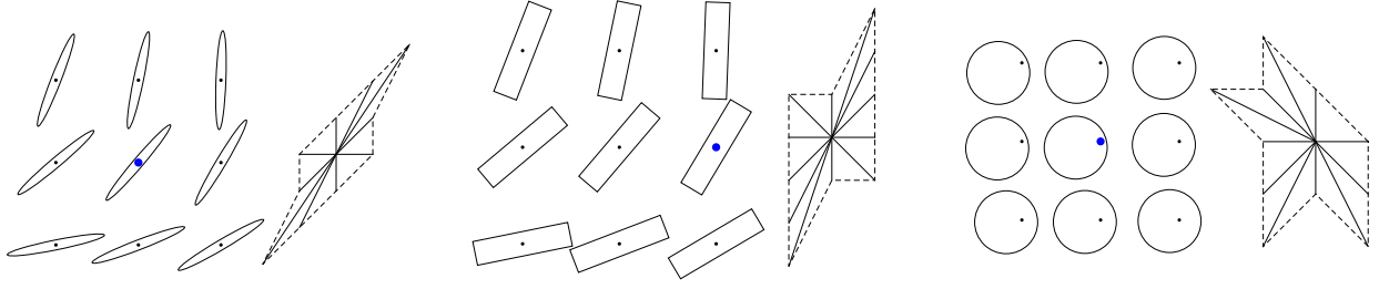
Figure 1: A Finsler metric \mathcal{F} , on a domain \Omega \subset \mathbb{R}^2 , is the data of a continuously varying asymmetric norm \mathcal{F}_z , at each point z \in \bar{\Omega} . The convex sets \{u; \mathcal{F}_z(u) \leq 1\} , at several points z \in \Omega , are used to visualize the metric \mathcal{F} . Finsler metrics can be of Riemannian type (left), symmetric (center), or asymmetric (right). The discretization of the Escape Time problem involves the construction of local stencils, three those produced by the FM-ASR are illustrated.
