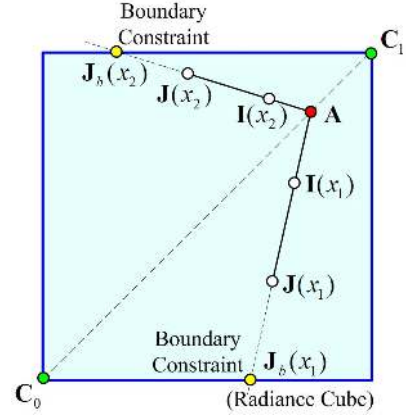
Figure 2. Radiance cube and boundary constraint. For each x , we require the extrapolation of \mathbf{J}(x) cannot cross over the boundary of the radiance cube. \mathbf{J}_b(x_1) and \mathbf{J}_b(x_2) are the corresponding boundary constraint points.
