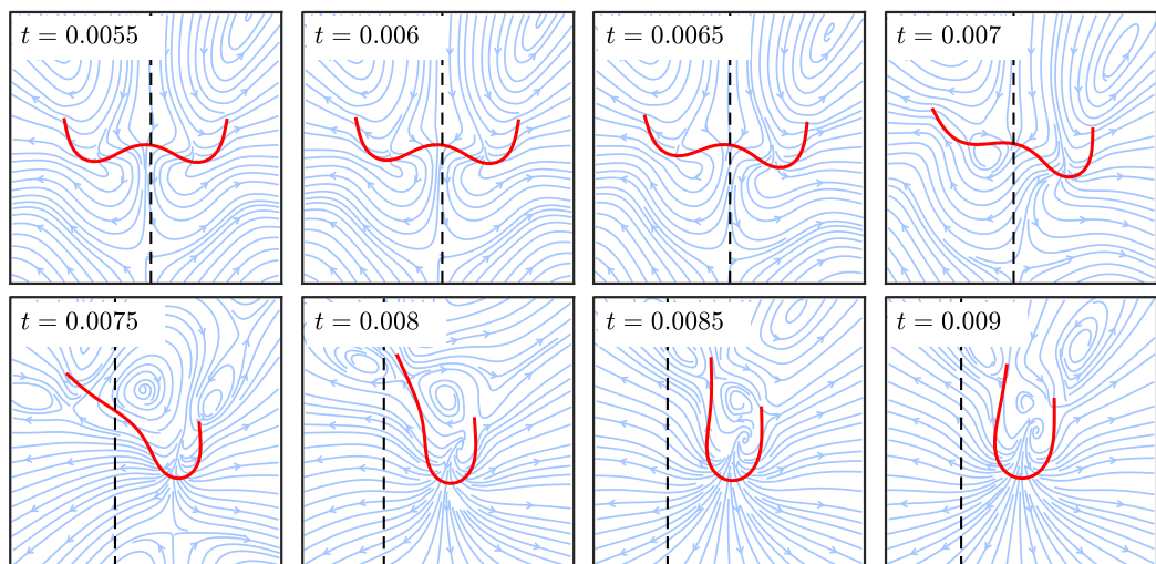
FIG. 7. Dynamics of a very flexible filament sedimenting under gravity. Here, for \mathcal{G} = 3500 , the filament first assumes a metastable “W” profile, before instability along the arclength transforms causes transition to the stable “U” configuration. In each panel, axes are centered on the center of gravity of the filament at the corresponding time point. The dashed line indicates the position of the center of gravity at t = 0 .
