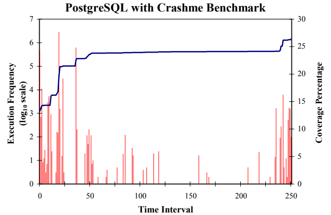
Figure 21. Instrumentation Code Execution Frequency and Source Code Line Coverage Percentage for PostgreSQL with Crashme Benchmark
