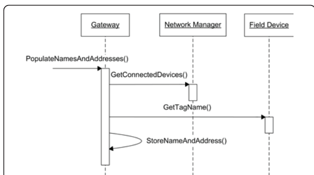
Figure 7 The WirelessHART gateway queries the network manager for a list of active WirelessHART devices. Using the list of active devices from the network manager, the gateway queries the active devices for their tag names. Now the gateway can map the device network address to a Profinet IO slot.
