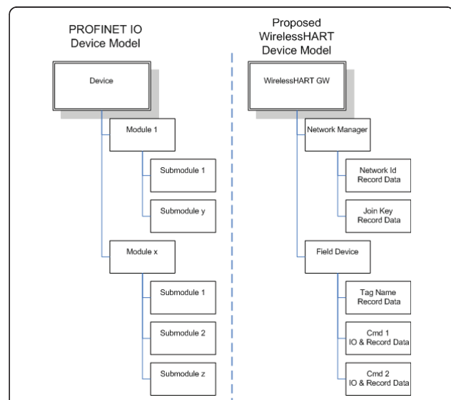
Figure 6 WirelessHART physical or logical devices are modeled as modules, and the module indicates the communication status of the device. WirelessHART functionality is modeled as submodules, which can communicate configuration data (Record Data Items) and/or process values (IO Data). The submodules can also indicate their status for additional status information.
