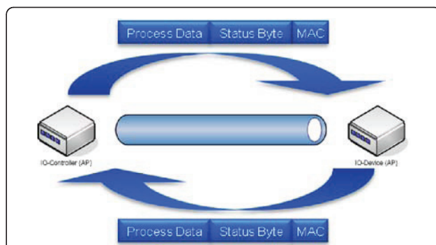
Figure 8 An example where security modules protect the integrity and authentication of the process data transmitted on Profinet IO.
