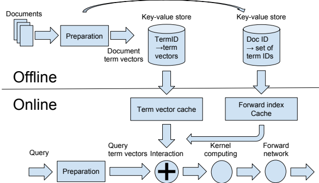
Figure 1: Architecture of interaction-based neural ranking.
