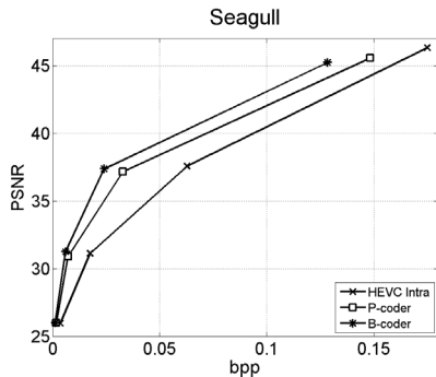
Fig. 7. PSNR over bpp for Seagull.
