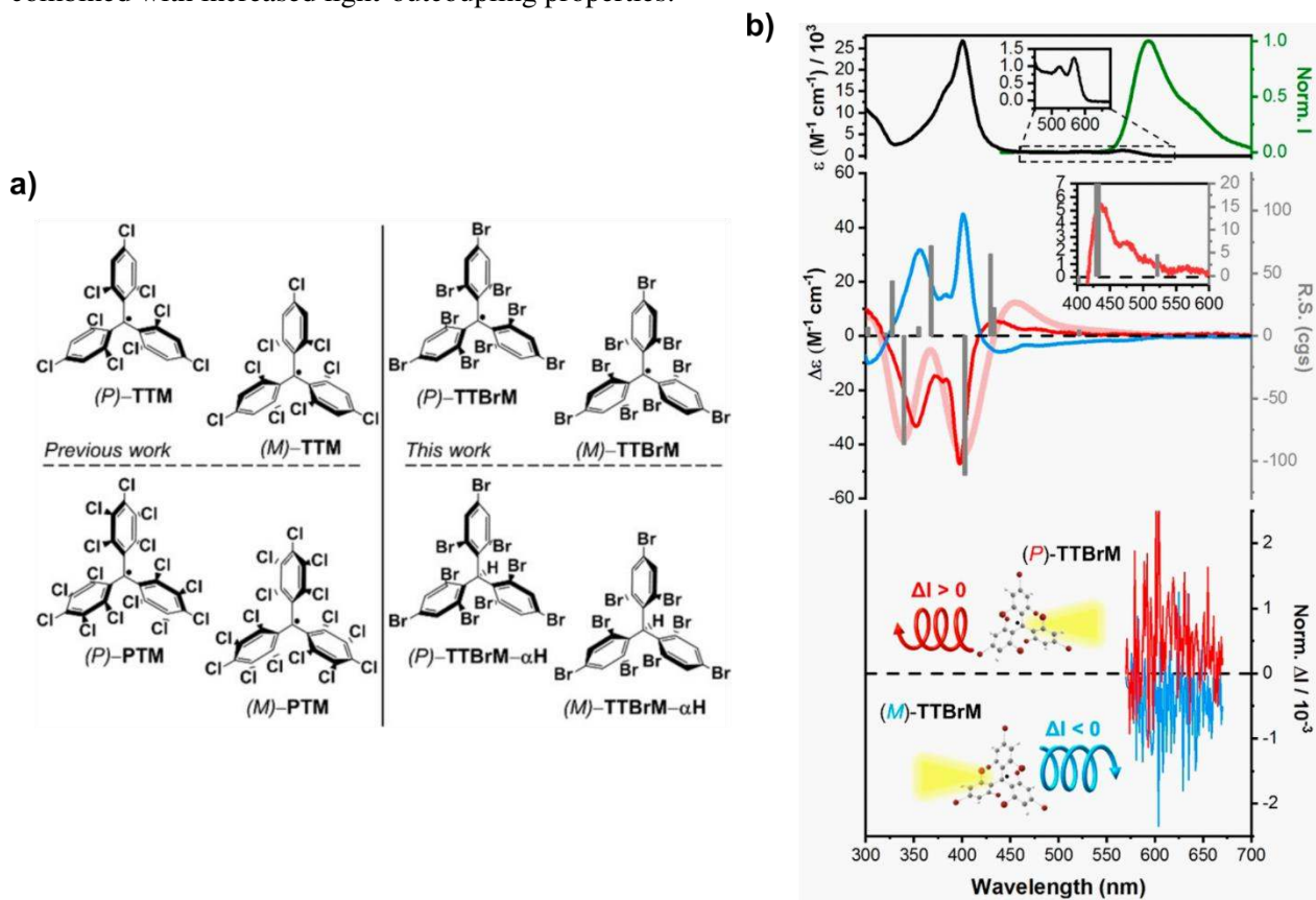
Fig. 10. Circularly polarised light emission
