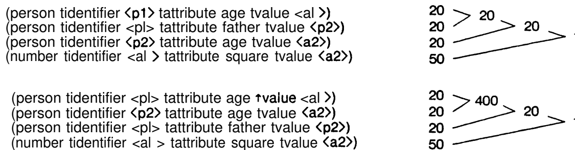
Figure 9-1: Illustration of the Cross-product Effect
