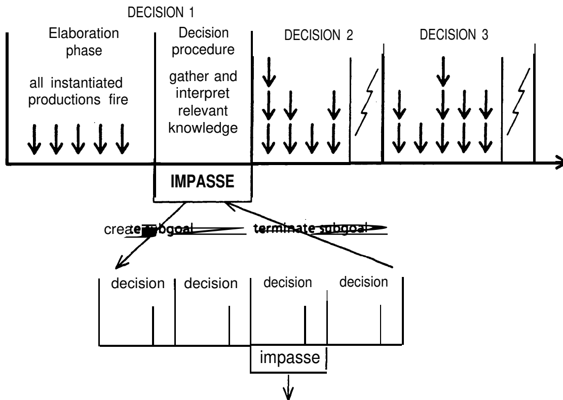
Figure 5-1: The SOAR Decision Cycle
