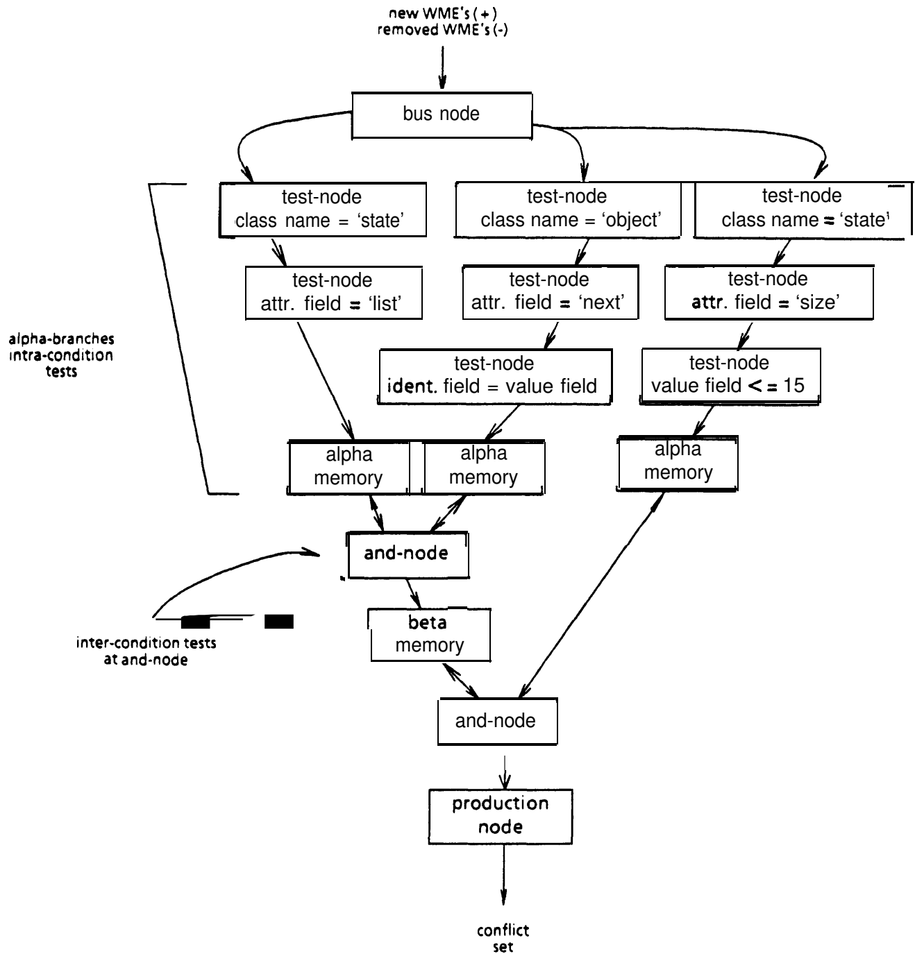
Figure 4- 1: Structure of a Small Rete Network
