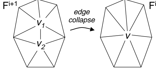
Figure 1: Edge collapse transformation.
