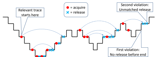
Figure 1. Example trace for structured acquire and release of locks
