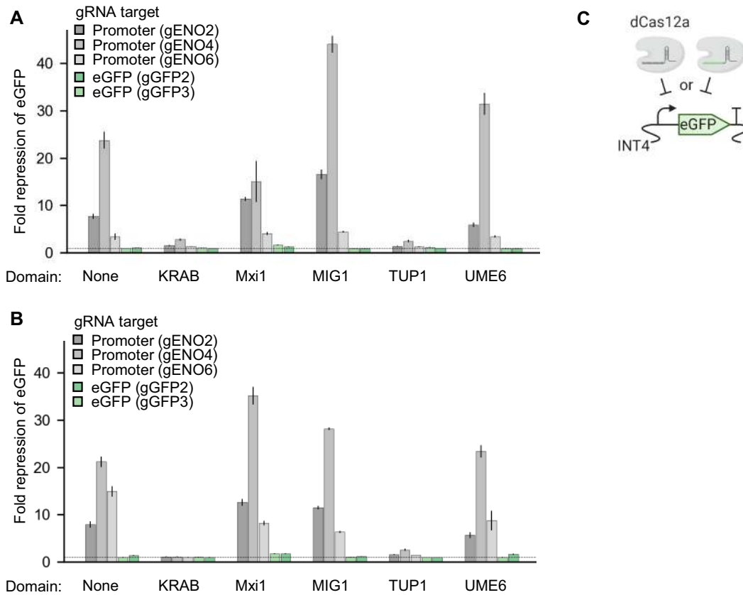
Figure 2. Comparison of repression domains and mutations defining nuclease-deficiency in dCas12a. (A). Downregulation efficiency of dCas12a D832A and repression domains genome integrated in strains DC002, DC004-008. (B). Downregulation efficiency of dCas12a E925A and repression domains genome integrated in strains DC003, DC009-013. Bars represent fold repression between targeting and non-targeting gRNA \pm 1 standard error ( n = 4 ). Dashed line indicates 1-fold change (i.e. no repression). (C). dCas12a variants were assessed in downregulation of genome integrated eGFP (locus INT4) in strains DC002-013 using gRNAs targeting the KIENO1 promoter or eGFP ORF.
