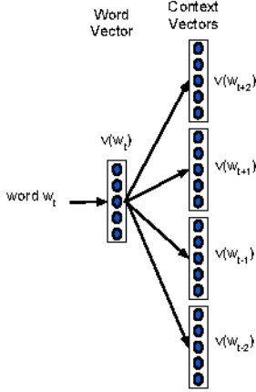
Figure 1: Architecture of the Skip-gram model with window size R_t = 2 . Context c_t of word w_t consists of w_{t-1}, w_{t-2}, w_{t+1}, w_{t+2} .
