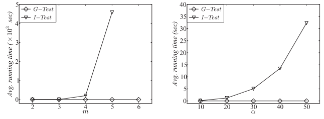
Fig. 15. Validation evaluation time
