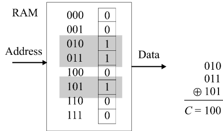
Fig. 3. Modulo-2 address characteristic for bit-oriented RAMs.
