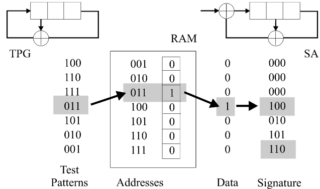
Fig. 5. Correspondence between signature analysis and modulo-2 address characteristic.
