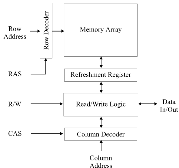
Fig. 2. Typical organization of a dynamic RAM.
