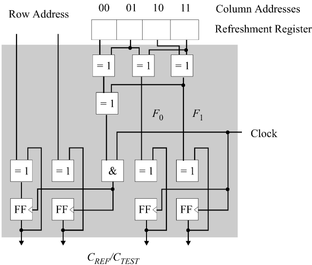
Fig. 8. Data compressor for the fast computation of row characteristics.
