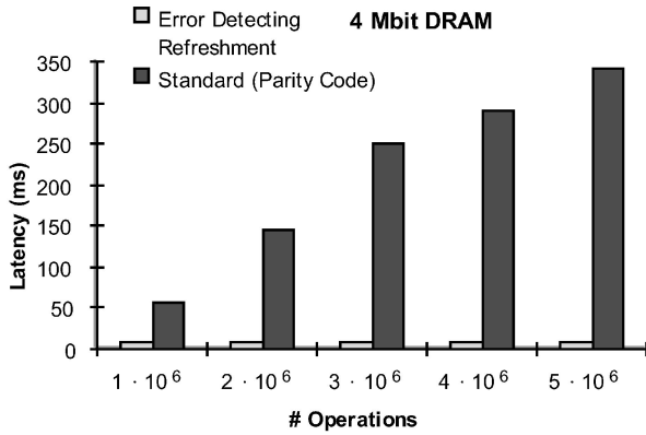
Fig. 10. Average error detection latency for a 4 Mbit DRAM.
