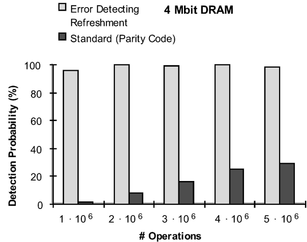
Fig. 11. Average detection probability for a 4 Mbit DRAM.
