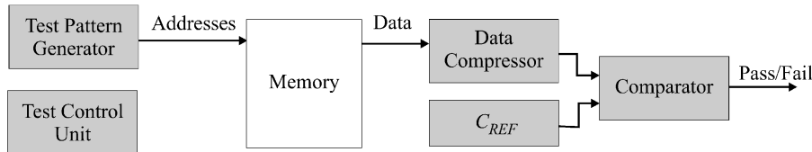
Fig. 1. Typical BIST architecture for memories.
