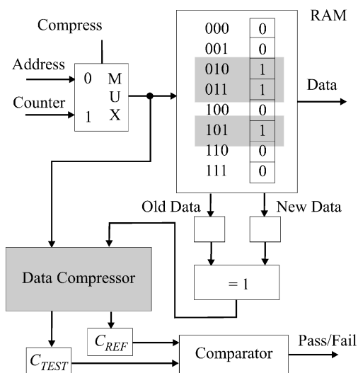
Fig. 4. Consistency checking based on the modulo-2 address characteristic.
