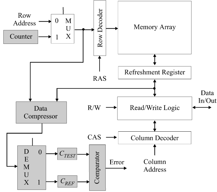
Fig. 9. Complete architecture for a DRAM with error detecting refreshment.
