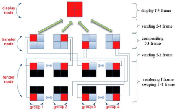
Fig. 3. Hybrid partition pipeline, k=2, n=4
