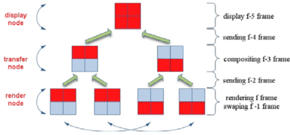
Fig. 2. Pipeline based on Binary Swap, n=4
