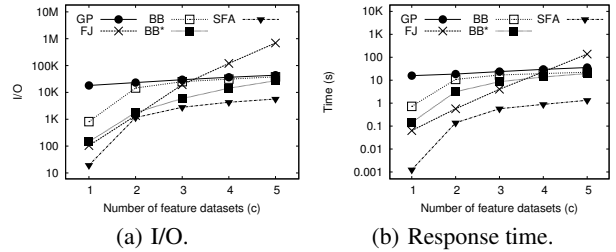
Figure 6: Effect of c on I/O and response time (range score).
