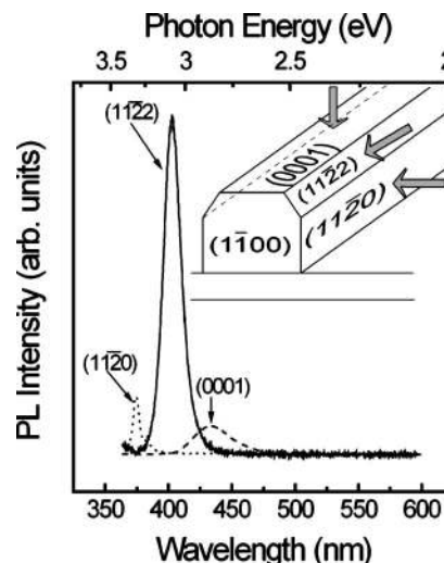
FIG. 2. Microscopic PL spectra from the (11\bar{2}0) , (11\bar{2}2) , and (0001) MQWs at RT. The inset figure shows the schematic sample structure, and arrows indicate the directions for excitation and collection.
