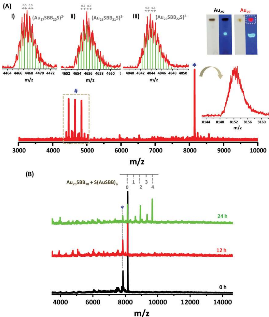
Fig. 2 ESI MS (A) and time dependent evolution of MALDI mass spectra (B) in negative ion mode of the red luminescent Au_{29} cluster. The three prominent peaks (marked with a #) apart from parent Au_{25}SBB_{18} (marked with a * and expanded to depict the isotopic distribution corresponding to -1 charge) are expanded in insets (i–iii). The green lines in (i–iii) are the simulated isotope patterns for (i) [Au_{27}(SBB)_{20}S]^{2-} , (ii) [Au_{28}(SBB)_{21}S]^{2-} , and (iii) [Au_{29}(SBB)_{22}S]^{2-} . Peak separation of m/z 0.5 is marked in the experimental spectra. The inset of (A) also shows the TLC separation of parent Au_{25} and the red luminescent Au_{29} cluster (marked with a dotted circle) eluted with a DCM/hexane mixture (80 : 20) as the eluent. Fragmentation due to the C–S cleavage of the SBB ligand from Au_{25} (marked with an asterisk in B) is also observed.
