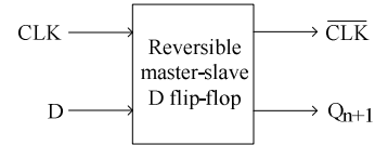
Fig. 13: Block diagram of reversible master-slave D flip-flop
