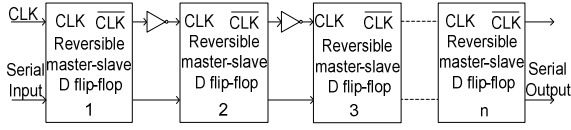
Fig. 14: Proposed reversible n-bit shift register
