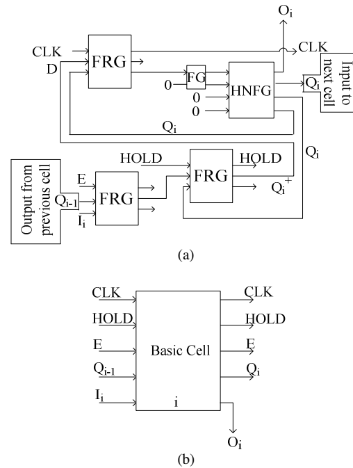
Fig. 16: Basic cell for the proposed reversible PIPO shift register: (a) Structure; (b) Block diagram
