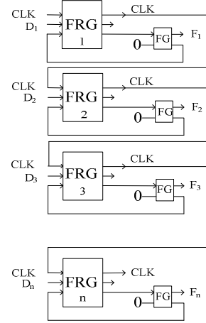
Fig. 11: Proposed n-bit reversible register
