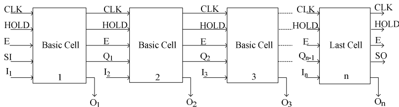
Fig. 17: Proposed reversible PIPO shift register using D flip-flops
