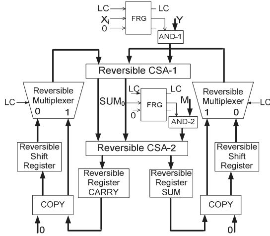
Fig. 19: Proposed architecture of reversible Montgomery multiplier
