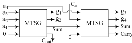
Fig. 9: Proposed four-to-two reversible CSA using MTSG gates
