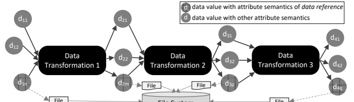
Fig 4. Synthetic workflow. The data values per transformation vary as in Table 1.
