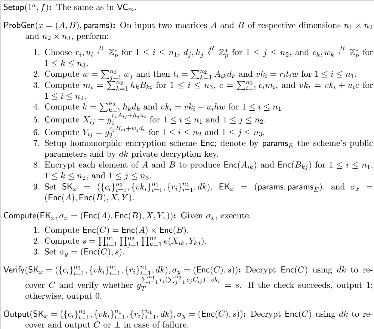
Figure 4: Description of scheme \text{VC}_m^p for malicious adversaries that achieves data privacy.
