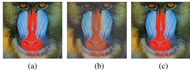
Figure 1. Example of binarized networks based on SRResNet [18], with a factor of 4 \times . (a) Real-weight network; (b) Fully-binarized network using binarization strategy [23]; (c) Our binarized network.
