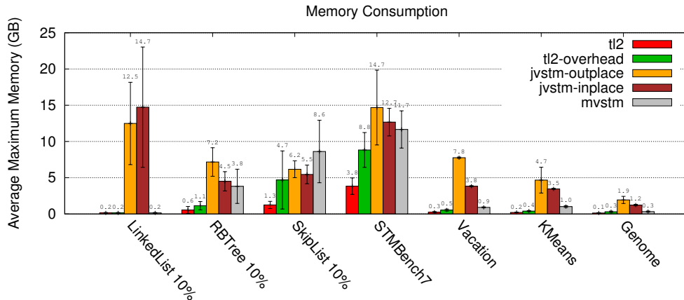
Figure 14: Maximum memory usage for each benchmark.
