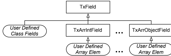
Figure 2: Metadata classes hierarchy.
