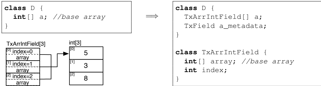
Figure 7: Memory structure of a TxArrIntField array.
