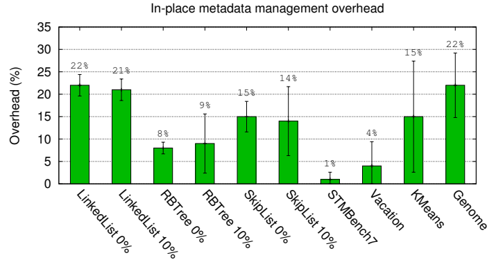
Figure 11: Performance overhead measure of the usage of metadata objects relative to out-place TL2.
