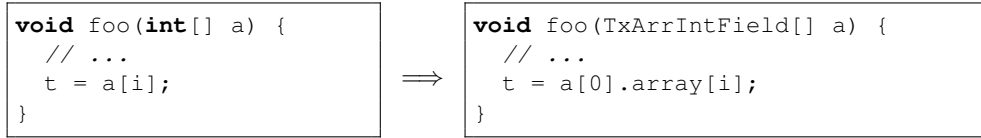
Figure 8: Example transformation of array access in the in-place strategy.
