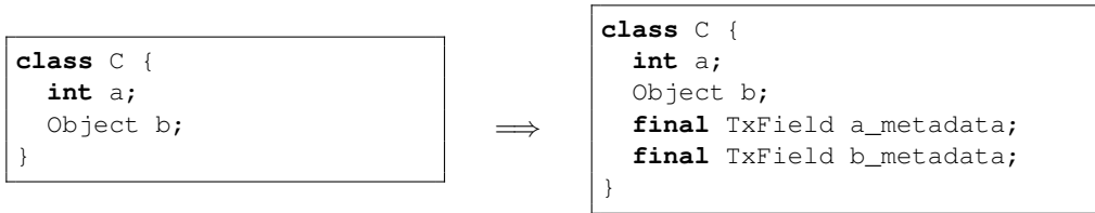
Figure 6: Example transformation of a class with the in-place strategy.
