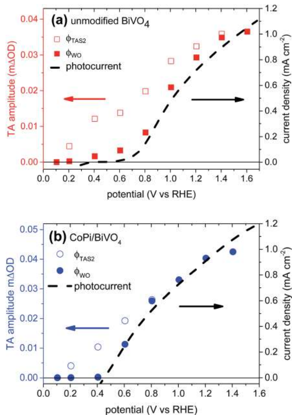
Fig. 6 Empty red squares and empty blue circles: transient absorption amplitude of long-lived holes ( \phi_{\text{TAS2}} ) in unmodified (a) and CoPi-modified (b) \text{BiVO}_4 photoanodes, obtained from eqn (2), as a function of applied potential. Filled red squares and filled blue circles: amplitude of holes that contribute to water oxidation ( \phi_{\text{WO}} ) in unmodified (a) and CoPi-modified (b) \text{BiVO}_4 photoanodes, calculated from eqn (4). The photocurrent data (dashed black lines) shown in these figures are directly compared in Fig. S2 in the ESI.†
