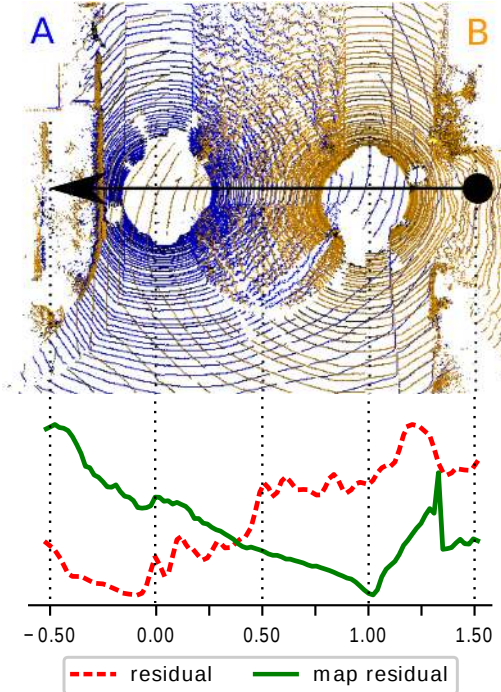
Fig. 5. Shown are two scans A (blue) and B (orange) from different sides of a street from KITTI sequence 06 from a birds eye view. From both sides, the other side’s street is not visible and therefore hard to distinguish the correct from the incorrect loop closure just by means of residual of an alignment. Shown below is the residual along the arrow, i.e. , at every position on the arrow we compute the residual from A to B if B would exactly lie at that position. Shown is the residual (red) of B to A and the map residual (green) of scan B to the composed virtual view .
