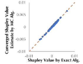
Figure 5: The SV produced by the exact algorithm and the baseline MC approximation algorithm.
