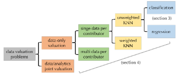
Figure 3: Classification of data valuation problems.
