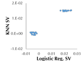
Figure 15: Comparison of the SV for a logistic regression and a KNN trained on the Iris dataset.
