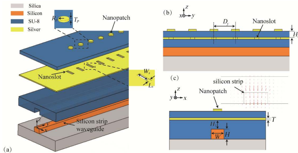
Fig. 1. Structure of the proposed nanopatch array. (a) Illustration of the structure layer by layer. (b) Side view of the device along the yz symmetric plane. (c) Cross-section view of the device. The inset shows the electric field distribution of the waveguide mode at 1550 nm. The parameters are as follows: W = 0.46 , H = 0.24 , H_1 = 0.3 and T = 0.08 , all in \mu\text{m} .
