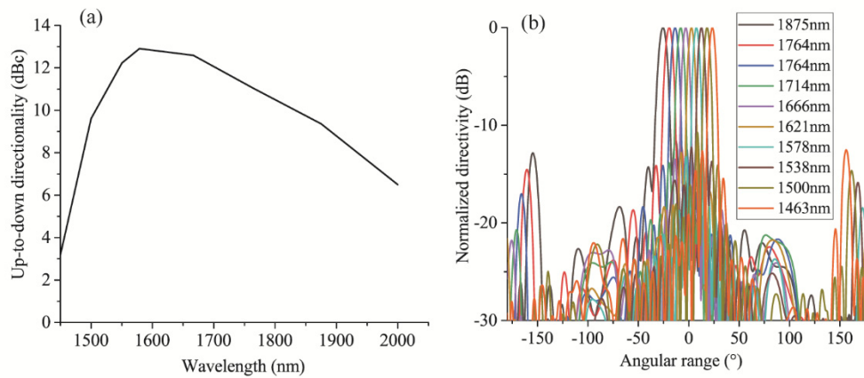
Fig. 7. (a) Up-to-down directionality versus wavelength. The parameters are the same as those in Fig. 3. (b) Normalized far-field directivity patterns at various wavelengths.
