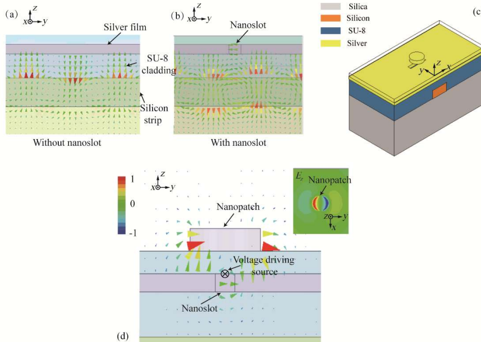
Fig. 2. (a) and (b). Electric field distributions of the hybrid plasmonic waveguide on the yoz plane with (b) and without (a) the nanoslot. The parameters are as follows: W = 0.46 , H = 0.24 , T = 0.08 , W_s = 0.4 , L_s = 0.1 and H_1 = 0.2 , all in \mu\text{m} . (c) Models used for single element simulation. The dimensions of the waveguide are the same as those in (b) and the other parameters are as follows: R_p = 0.18 , H_2 = 0.1 and T_p = 0.1 , all in \mu\text{m} . The SU-8 substrate between the nanopatch and the silver thin film is set to be transparent to clearly show the nanoslot. (d) Electric field distributions on the yoz plane for the model in (c). The inset shows the E_z distribution on the bottom surface of the nanopatch. In the simulation, a voltage driving source is placed on the top of the nanoslot to excite the nanopatch. The wavelength is 1550 nm.
