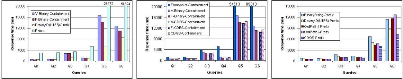
(a) Response time of different schemes (b) Response time of containment schemes (c) Response time of prefix schemes
