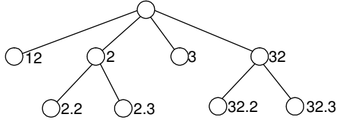
Fig. 9 CDQS-Prefix scheme (for Figure 3)
