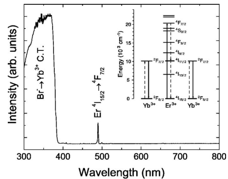
FIG. 3. Excitation spectrum of \text{Cs}_3\text{Y}_2\text{Br}_9:1\%\text{Er}; 15\%\text{Yb} for \text{Yb}^{3+} {}^2\text{F}_{7/2} emission at 999 nm. T=4.4 K. The inset shows the energy level diagrams of \text{Er}^{3+} and \text{Yb}^{3+} and the downconversion process is depicted. Broken lines indicate energy transfer while the drawn lines depict radiative decay.
