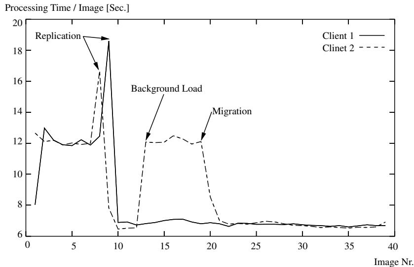
Fig. 7. The load managed medical image-processing application.
