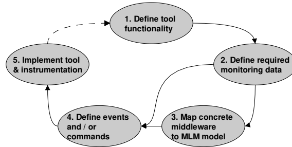
Fig. 4. MIMO tool development methodology.
