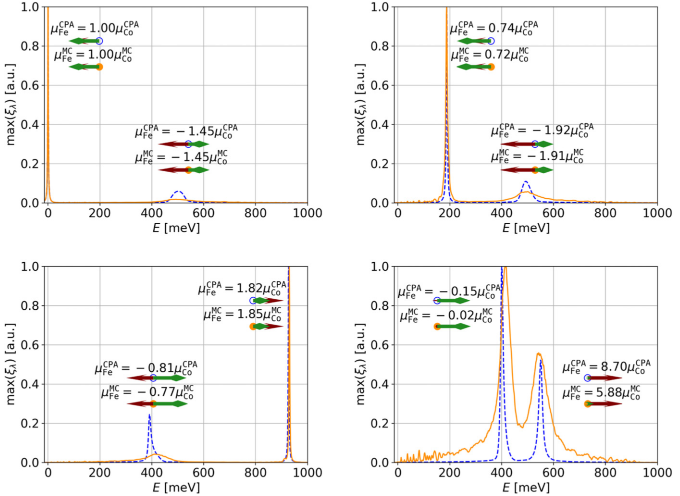
Figure 5. Maximal eigenvalue of the loss matrix at \Gamma (top left), \frac{\Gamma_3}{3} (top right), H (bottom left) and N (bottom right). All results are calculated at T = 0 K within the MC (orange solid line) and CPA (blue dashed line). The spatial shape of the modes is drawn near the peaks. Starting from a blue empty circle (CPA) or an orange filled circle (MC), the magnetic moments of iron are drawn as brown pointy vectors while the moments of cobalt are visualized as green edgeless vectors.
