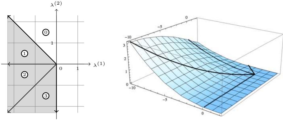
Fig. 4. a Chambers and support (gray) and b density function of the iterated convolution computed in Lemma 5.9
