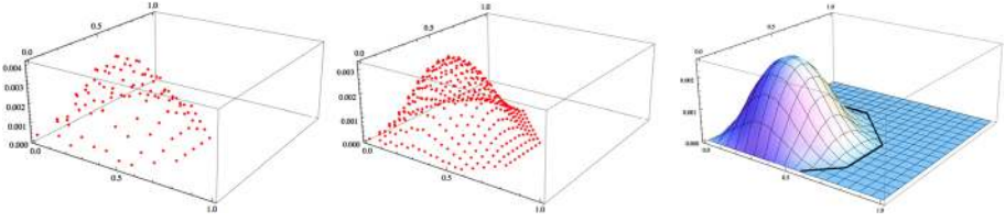
Fig. 7. a, b Illustration of the multiplicity measures \mu_{M,k}^K for the mixed-state quantum marginal problem of two qubits with global spectrum (4/7, 2/7, 1/7, 0) and k = 28, 56 , which have been computed by the algorithm described in Sect. 7.1. c Their semi-classical limit, i.e., the corresponding Duistermaat–Heckman measure as computed in Sect. 5.2
