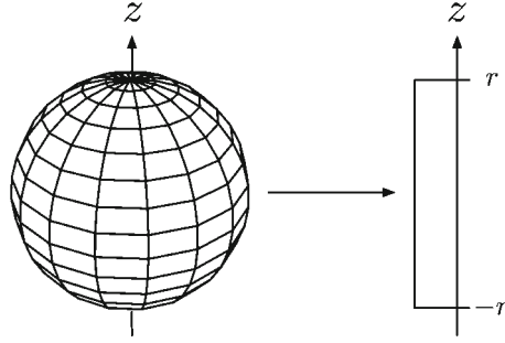
Fig. 1. A Bloch sphere, its height function and the induced measure: a generic coadjoint SU(2) -orbit, its Abelian moment map and the Abelian Duistermaat–Heckman measure
