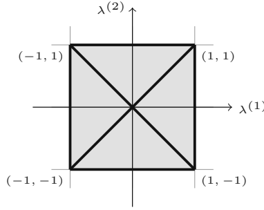
Fig. 2. Abelian moment polytope of two qubits (grey square) and its decomposition into four bounded regular chambers by the critical walls (thick lines)
