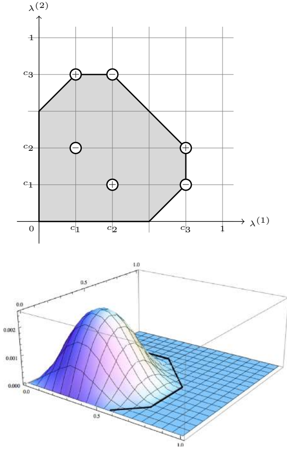
Fig. 5. a Non-Abelian moment polytope (gray), and the points \pi(\tilde{w}\tilde{\lambda}) \in \mathfrak{t}_+^* together with \text{sign}(\tilde{w}) . b Density of the Duistermaat–Heckman measure for global spectrum (4/7, 2/7, 1/7, 0)
