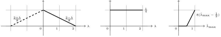
Fig. 6. a, b Density of the Abelian and the non-Abelian Duistermaat–Heckman measure for \mathbb{P}(\text{Sym}^2(\mathbb{C}^2)) , and c corresponding maximal eigenvalue distribution of the one-body reduced density matrix
