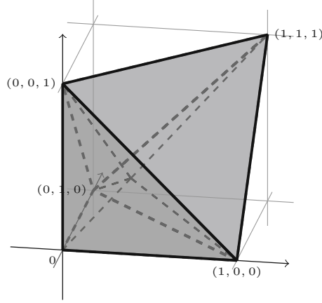
Fig. 3. Non-Abelian moment polytope of three qubits and its decomposition into domains of polynomiality for the non-Abelian Duistermaat–Heckman measure. Each domain is the union of two regular chambers
