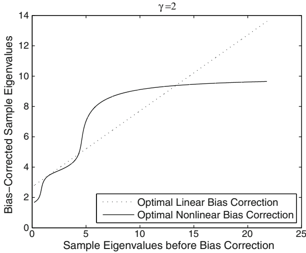
Fig. 3 Comparison of the optimal linear versus nonlinear bias correction formulæ. In this example, the distribution of population eigenvalues H places 20% mass at 1, 40% mass at 3 and 40% mass at 10. The solid line plots \delta(\lambda) as a function of \lambda
