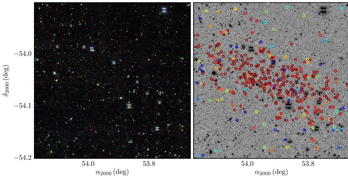
Figure 2. Left: false color gri coadd image of the 0^{\circ}.3 \times 0^{\circ}.3 region centered on DES J0335.6–5403. Right: stars in the same field of view with membership probability p_i > 0.01 are marked with colored circles. In this color map, red signifies high-confidence association with DES J0335.6–5403 and blue indicates lower membership probability. The membership probabilities have been evaluated using Equation (2) for the best-fit model parameters listed in Table 1.
