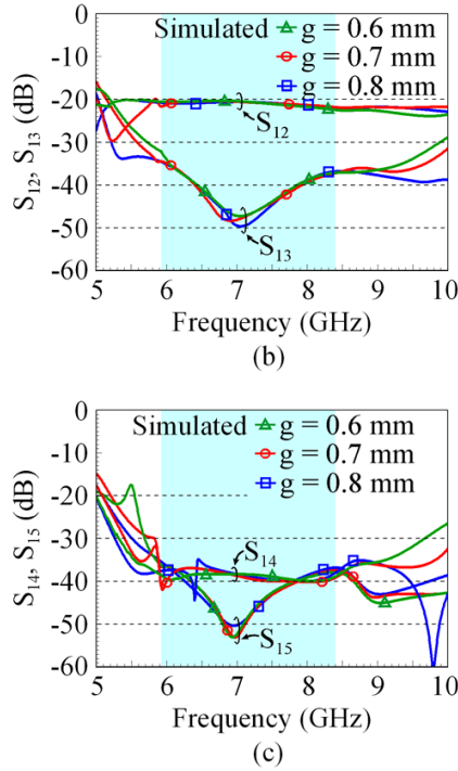
FIGURE 16. Simulated S parameters of Port P1 as a function of the feed gap ( g ). (a) S_{11} . (b) S_{12} ( = S_{18} ), S_{13} ( = S_{17} ). (c) S_{14} ( = S_{16} ), S_{15} . Other parameters are same as in Fig. 1.
