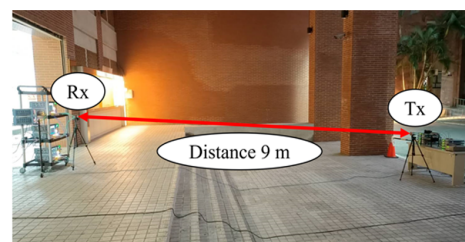
FIGURE 28. The 8 x 8 MIMO testing with Tx outdoor/Rx indoor scenario in the open concave space in front of the entrance of the EE department building, NSYSU. (a) Panoramic view for two orientations with Tx fixed (Rx LOS to Tx and Rx non-LOS to Tx). (b) Setup positions for Rx LOS to Tx; Rx non-LOS to Tx also with a distance of 9 meters.
