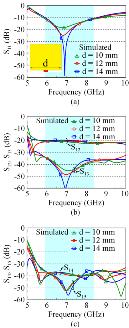
FIGURE 14. Simulated S parameters of Port P1 as a function of the planar monopole width ( d ). (a) S_{11} . (b) S_{12} ( = S_{16} ), S_{13} ( = S_{17} ). (c) S_{14} ( = S_{16} ), S_{15} . Other parameters are same as in Fig. 1.
