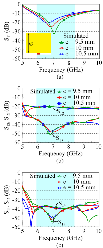
FIGURE 15. Simulated S parameters of Port P1 as a function of the planar monopole length ( e ). (a) S_{11} . (b) S_{12} ( = S_{16} ), S_{13} ( = S_{17} ). (c) S_{14} ( = S_{16} ), S_{15} . Other parameters are same as in Fig. 1.
