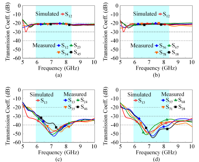
FIGURE 19. Measured transmission coefficients. (a) Two adjacent ports ( S_{12} , S_{23} , S_{34} , S_{45} ). (b) Two adjacent ports ( S_{56} , S_{67} , S_{78} , S_{18} ). (c) Two ports spaced by one planar monopole ( S_{13} , S_{24} , S_{35} , S_{46} ). (d) Two ports spaced by one planar monopole ( S_{57} , S_{68} , S_{71} , S_{28} ).
