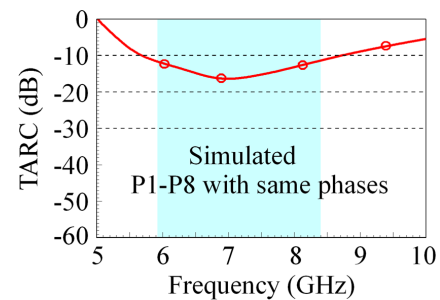
FIGURE 7. Simulated total active reflection coefficient (TARC) of Ports P1-P8 excited with same excitation phases in the MIMO array.
