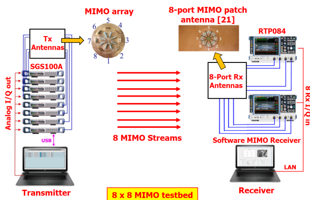
FIGURE 27. The 8 x 8 MIMO testbed at National Sun Yat-sen University (NSYSU) [2]. The fabricated MIMO array is applied as the transmit (Tx) antennas. The 8-port MIMO patch antenna [21] is used as the receive (Rx) antennas at the receiver.
