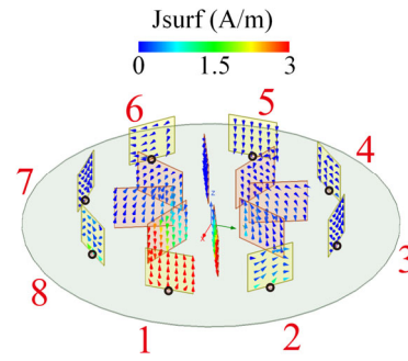
FIGURE 3. Simulated vector surface current distributions of Port P1 excited at 7.1 GHz with Ports P2-P8 terminated to 50 Ω.
