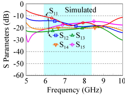
FIGURE 9. Simulated S parameters of Port P1 in the MIMO array without the radial metal walls.
