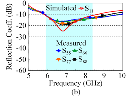
FIGURE 18. Measured reflection coefficients. (a) Ports P1-P4. (b) Ports P5-P8.
