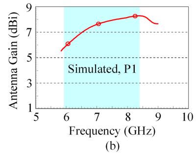
FIGURE 6. Simulated (a) antenna efficiency and (b) antenna gain of Port P1 in the MIMO array.
