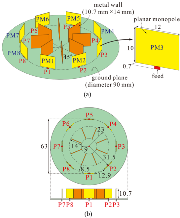
FIGURE 1. Geometry of the simple planar monopole MIMO circular array (PM1-PM8 with Ports P1-P8) for 6G upper mid-band 8 x 8 MIMO access points. (a) Perspective view. (b) Top and side views.
