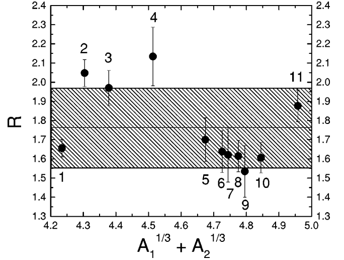
FIG. 4. Ratio between the reduced values of the “elastic fission” and the fusion barriers, R = v_{ef} / v_{fus} , for the systems investigated in the present work as a function of the size of the system A_1^{1/3} + A_2^{1/3} . The hatched lines represent the average value for R and their width represents its uncertainty. The numbers represent the following systems: (1) {}^9\text{Be} + {}^{10}\text{B} , (2) {}^9\text{Be} + {}^{11}\text{B} , (3) {}^{10}\text{B} + {}^{11}\text{B} , (4) {}^{11}\text{B} + {}^{12}\text{C} , (5) {}^{16}\text{O} + {}^{10}\text{B} , (6) {}^{17}\text{O} + {}^{10}\text{B} , (7) {}^{16}\text{O} + {}^{11}\text{B} , (8) {}^{18}\text{O} + {}^{10}\text{B} , (9) {}^{17}\text{O} + {}^{11}\text{B} , (10) {}^{18}\text{O} + {}^{11}\text{B} , and (11) {}^{19}\text{F} + {}^{12}\text{C} .
