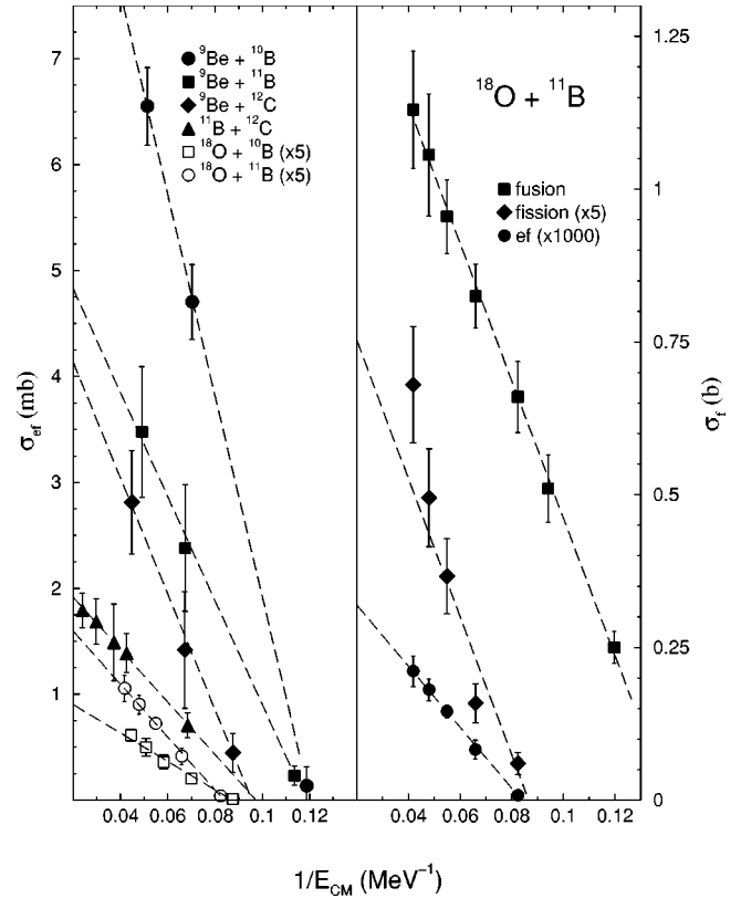
FIG. 2. Left: excitation function of the "elastic fission" yields for some systems. The dotted lines represent linear fits to the data points. Right: excitation function for the fusion [5], fission [5], and "elastic fission" yields for the ^{18}\text{O} + ^{10}\text{B} reaction.
