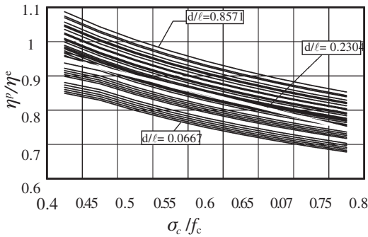
FIG. 8. (\frac{\eta_p}{\eta_e} - \frac{\sigma_c}{f_c}) curves for different values of d/l [4].
