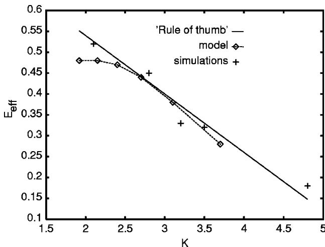
FIG. 4. E_{eff} as a function of K : the values given by Eq. (4) (model), published finite element method simulations (simulations), and the “rule of thumb” of Ref. [5].
