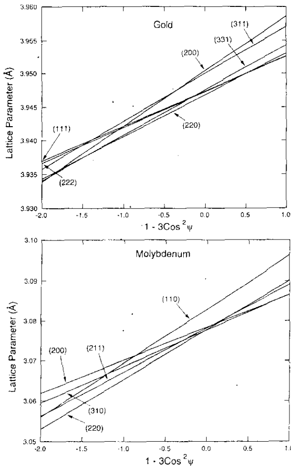
FIG. 4. Variation of lattice parameter determined from each diffraction line with angle for (a) gold and (b) molybdenum at 21.0 GPa. The solid lines are from the least-squares fits to d spacing versus 1 - 3 \cos^2 \psi (Fig. 3). The relative y-axis range in (b) is twice the relative y-axis range is (a).
