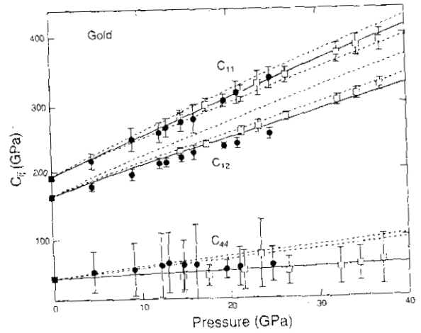
FIG. 9. Second-order elastic moduli of gold as a function of pressure. Filled circles are from this study. Open squares are from a rhenium/gold sample studied using the same technique (see Ref. 26). Error bars are one standard deviation. Solid lines are finite strain fits to the present data combined with it of Ref. 26 and ambient pressure data (see Ref. 17). The dashed lines show finite strain extrapolations of ultrasonic data (see Refs. 16 and 17), where the upper dashed curve corresponds to Ref. 16, and the lower dashed curve is from Ref. 17. The difference between adiabatic and isothermal moduli has been neglected.
