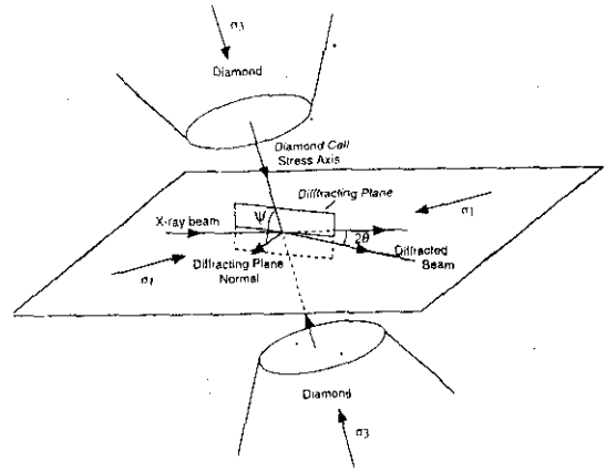
FIG. 1. Experimental geometry for radial diffraction experiments. \psi is the angle between the diamond cell stress axis and the diffraction plane normal.
