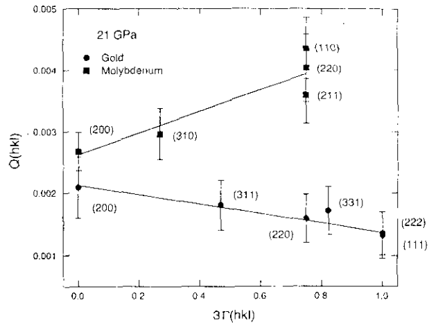
FIG. 6. Q(hkl) as a function of 3\Gamma for gold and molybdenum at 21.0 GPa. The solid lines are least-squares fits to the data. The estimated errors on Q(hkl) are obtained from the scatter of the d(hkl) vs 1 - 3 \cos^2 \psi relation.
