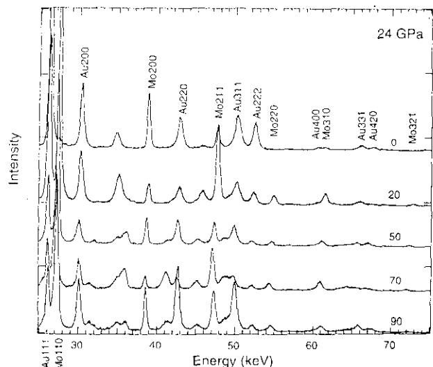
FIG. 2. Selected x-ray diffraction patterns as a function of angle from the stress axis at 24 GPa. Diffraction lines from molybdenum and gold are labeled. Unlabeled lines are from the beryllium gasket. The angle \psi , corresponding to each pattern, is shown at the right.
