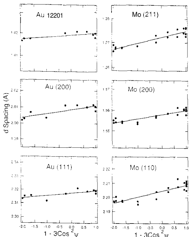
FIG. 3. Dependence of d spacing on 1 - 3 \cos^2 \psi for selected diffraction lines of gold and molybdenum at 9 GPa. The solid lines are least-squares fits to the data. The y-axis range is \pm 1\% for each panel.
