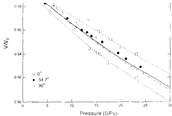
FIG. 7. Equation of state of molybdenum from lattice parameters measured at 0°, 54.7°, and 90°. The pressure is determined from the mean lattice parameter of gold. The dashed lines show Birch–Murnaghan equation fits to the data at 0° and 90°. The solid line shows the 300 K isotherm from ultrasonic data (Ref. 9), the dash-dot line shows the isotherm from high-pressure shock data (see Ref. 7), and the pluses are low-pressure shock data (see Ref. 12).
