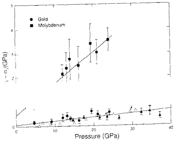
FIG. 8. Uniaxial stress component of gold (filled circles) and molybdenum (filled squares) as a function of pressure. Solid lines are least-squares fits to the data. For gold, open triangles are from Ref. 35 and filled triangles are from earlier radial diffraction data (see Ref. 26). For molybdenum, open symbols are yield strength measurements under shock compression (see Ref. 12).
