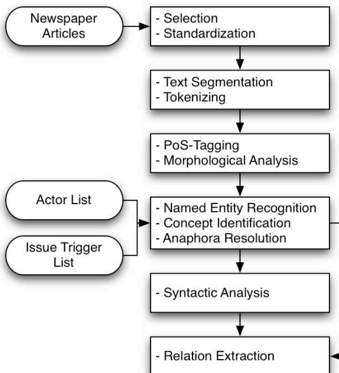
Figure 1: Software pipeline
