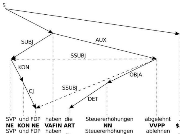
Figure 2b: Dependency tree with secondary relations
