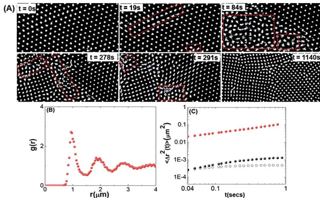
Fig. 7 (A) Time evolution of the 2D particle trajectories in the XY-plane over 300 frames ( =6 s) at \phi_{\text{eff}} = 0.66 after the application of an electric field at E = 0.045 V_{\text{rms}} \mu\text{m}^{-1} . Also shown is the corresponding structure with the pair correlation function g(r) (B) and the dynamics represented by the mean square displacement \langle \Delta r^2(t) \rangle (C) calculated in the disordered region at t = 84 s, respectively. In (C), the mean square displacement, \langle \Delta r^2(t) \rangle (red circles) calculated in the disordered region, is compared with that of \langle \Delta r^2(t) \rangle from a FCC (black open circles) and BCT crystalline state (black filled circles), respectively.
